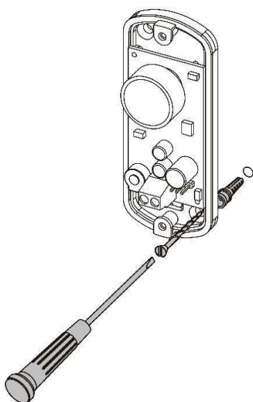
Figure 6.3 – Step 3: Mounting the EMFP on the wall.
