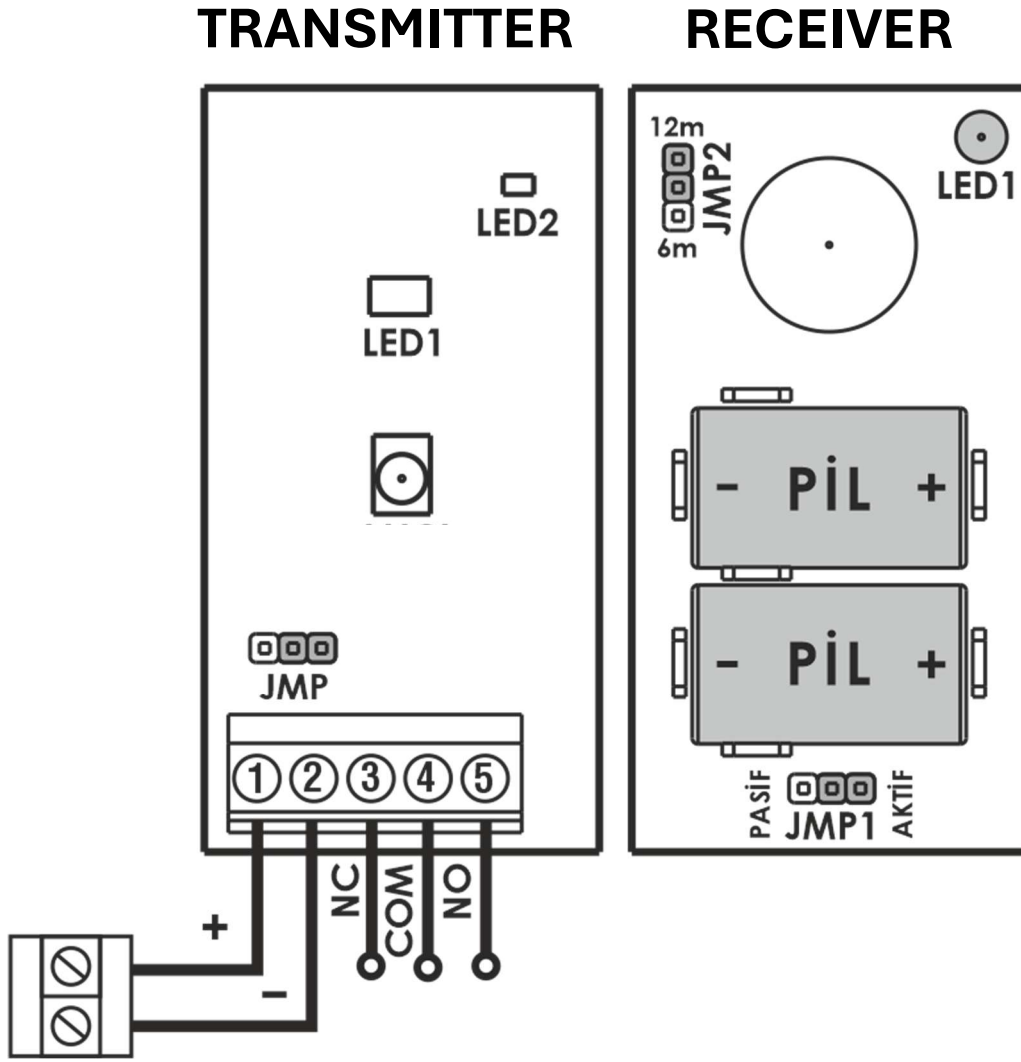
Figure 7.1 EMFP Wiring Diagram
