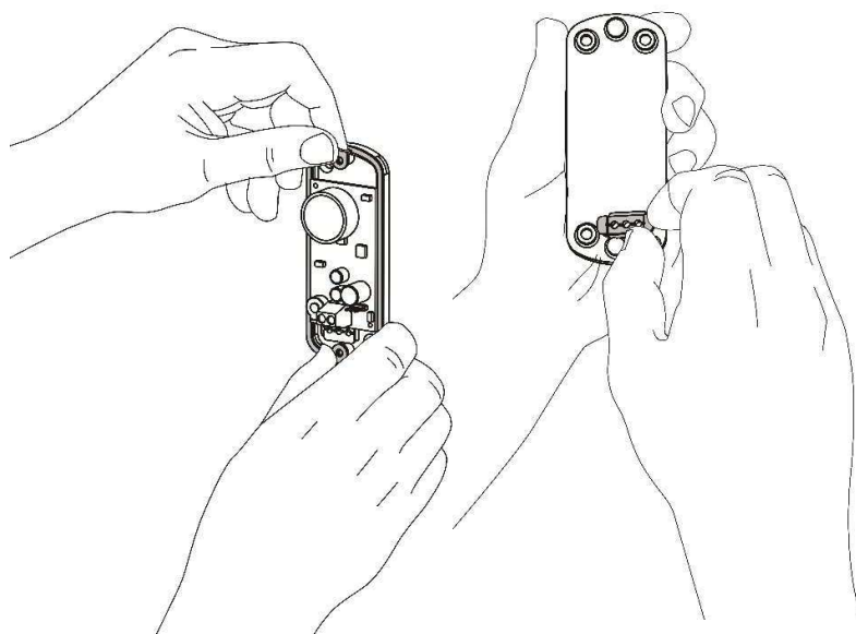
Figure 6.2 – Step 2: Installing the waterproof and protective seals on the EMFP.
