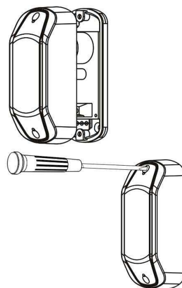
Figure 6.5 – Step 5: Reinstalling the front cover of the EMFP.
