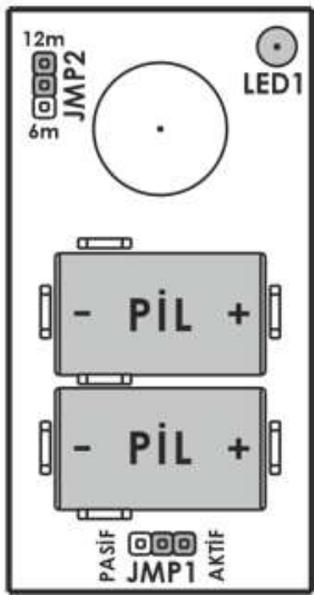
Figure 4.1 EMFP-V Control Board
