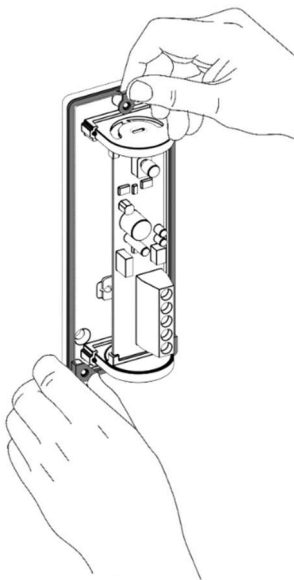
Figure 6.4 – Installing the internal waterproof gasket of the HFBM.
