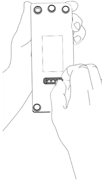
Figure 6.2 – Installing the rear waterproof gasket of the HFBM.
