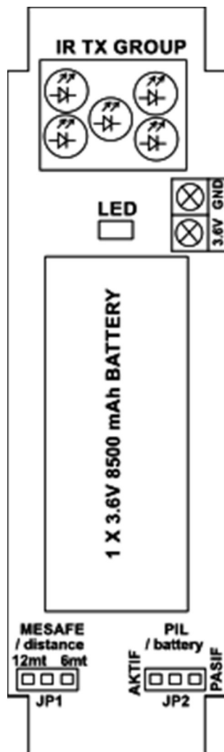
Figure 4.1 HFBM-V Control Board
