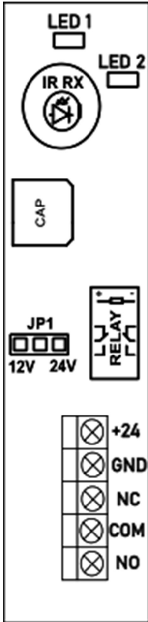
Figure 5.1 HFBM-A Control Board
