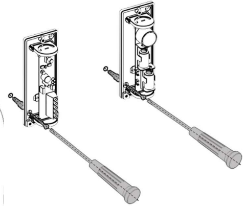
Figure 6.3 – Securing the HFBM to a flat surface with screws.
