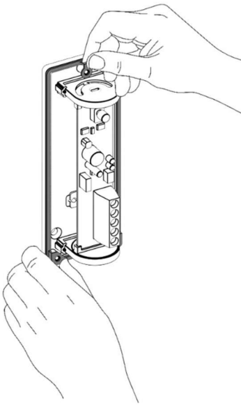
Figure 6.4 – Installing the internal waterproof gasket of the HFBM.
