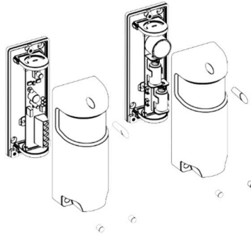
Figure 6.2 – Installing the rear waterproof gasket of the HFBM.
